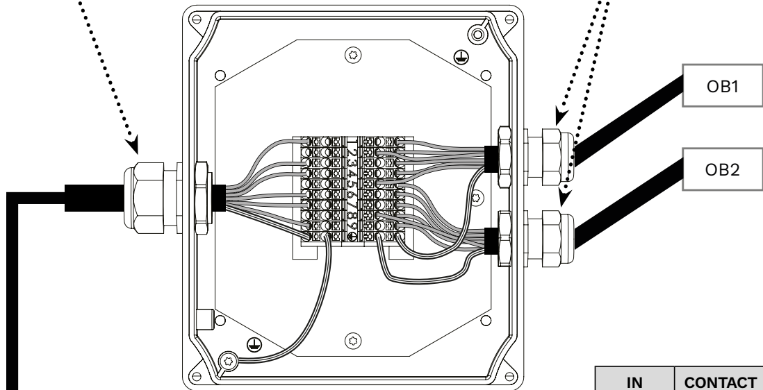
Connections inside Junction box
