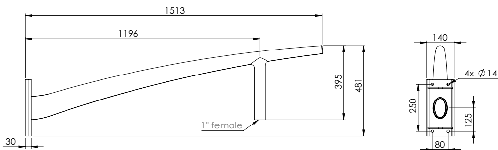
BOREAL Bracket lateral
