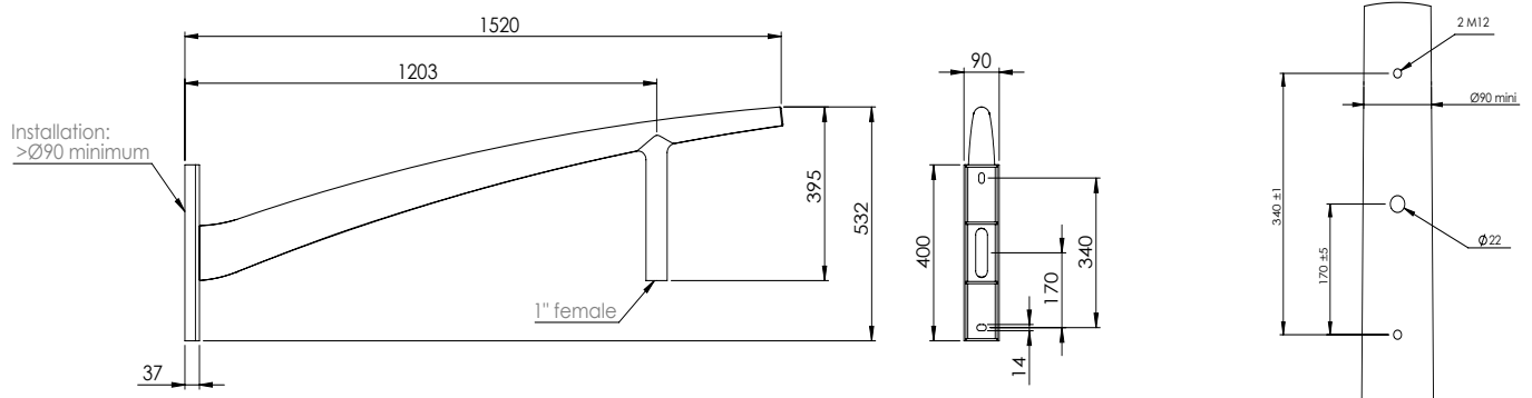
Drilling information for installation on pole
